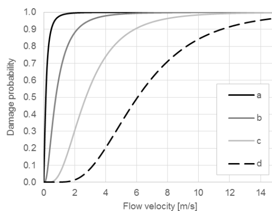
Fig. 3.8 Fragility curves admitted for road infrastructure
